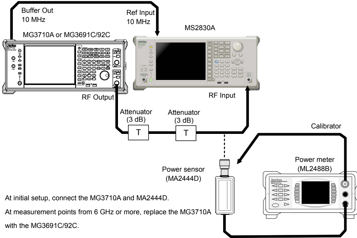
Figure 6.2.4-1 RF frequency characteristics test
