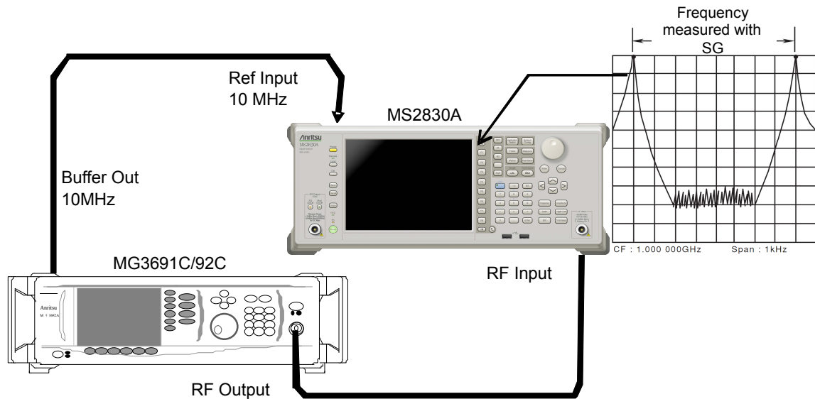
Figure 6.2.2-1 Frequency span display accuracy test
