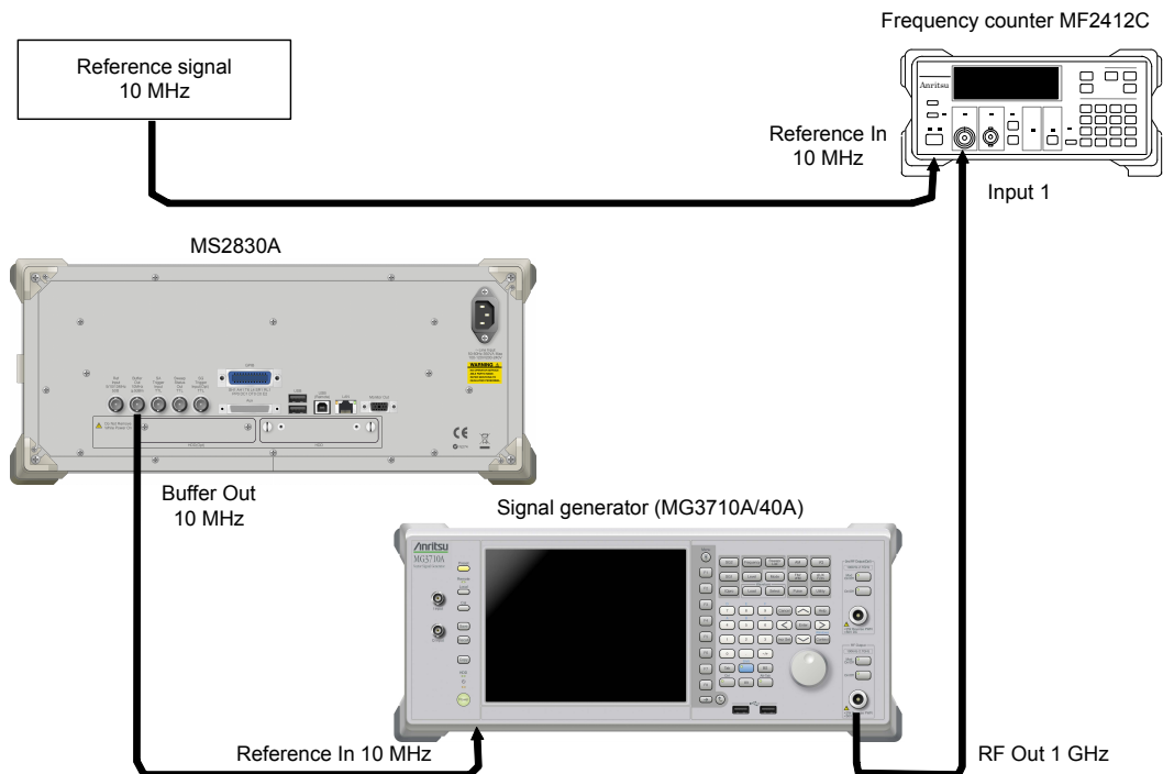
Figure 9.3.3-1 Connections for frequency calibration using frequency counter
