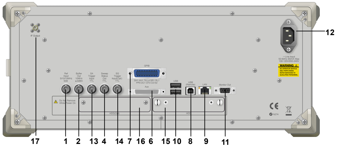
Figure 3.1.1-2 Rear panel
