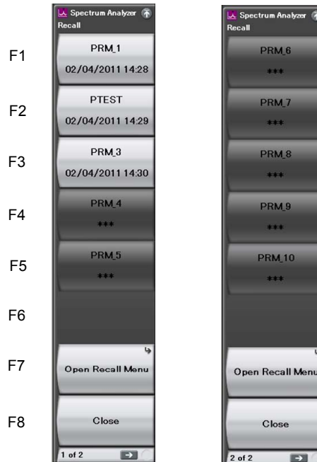
Figure 3.6.4-4 Simple Recall function menu
