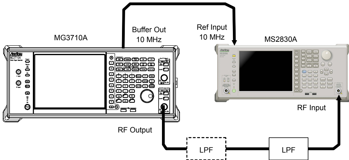
Figure 6.2.6-1 Second harmonic wave distortion test
